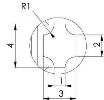
DETAIL D SCALE 10 : 1
